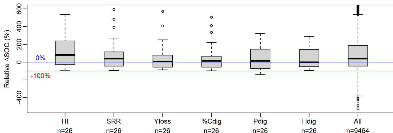
FIGURE 6 Simulated difference in SOC stocks between AD and no-AD scenarios with alternative parameter values relative to the simulated difference in SOC stocks between AD and no-AD scenarios with the reference parameter values (Relative \Delta SOC). Each boxplot represents the distribution of simulated values for all case studies together according to the different parameter values. \%C_{\text{dig}} , C remaining in digestate; All, all uncertainties together; H_{\text{dig}} , humification coefficient of the digestate; HI, harvest index; P_{\text{dig}} , proportion of digestate returned to soil; SRR, shoot:root ratio; Y_{\text{loss}} , yield loss of the primary crop following winter energy cover crop. A Relative \Delta SOC lower than -100\% indicates a decrease in SOC stocks in comparison with the non-AD scenario. Very few data are higher than 600\% (577 over 9620), and the y-axis is cut to 600\% to improve the visibility. AD, anaerobic digestion; SOC, soil organic carbon.
