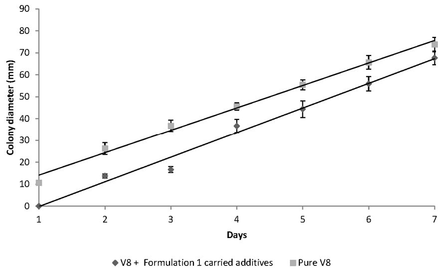
Figure 2. Effect of the carrier additives of formulation 1 on mycelial growth of P. megakarya
