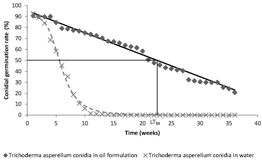
Figure 1. Germination level of T. asperellum conidia over time for formulated (◆) and non-formulated conidia (×) of T. asperellum PR11
