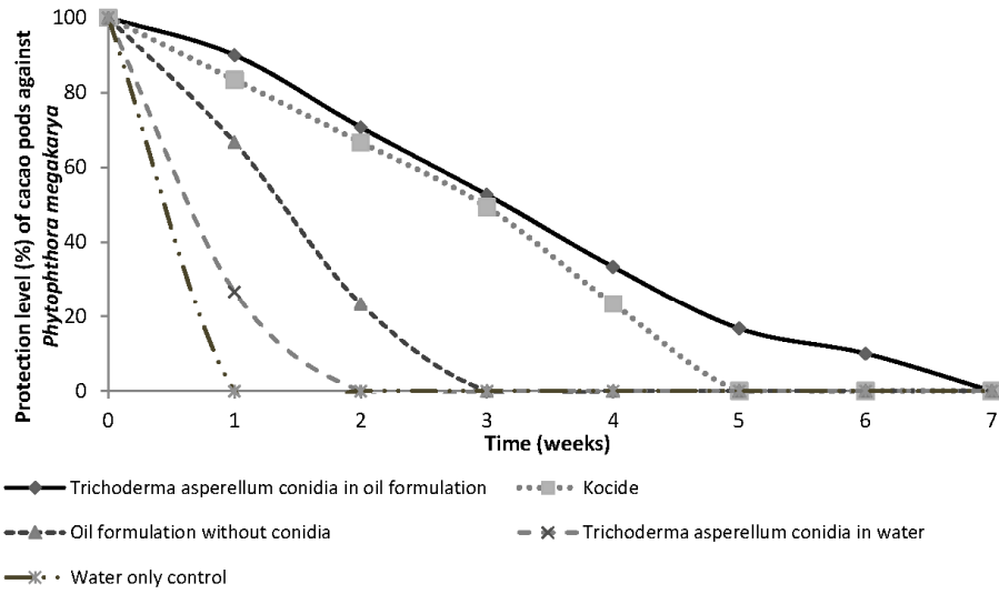
Figure 3. Protective effect over time of formulation 1 (◆) on cacao pods in the field compared with a fungicide (■), the formulation without conidia (▲), conidia in aqueous suspension (×) and a water only control (✱).
