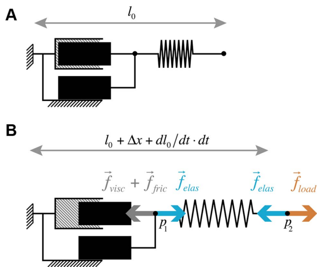
Fig. 8. 1D version of a unit element of the biomechanical model. a) the system in its resting configuration ( B_0 ). b) the system deformed by a the loading forces, at mechanical equilibrium ( B_1 ). Orange, blue and gray arrows represent respectively the loading (turgor-related) force, the elastic forces and the sum of viscous drag and friction force.
