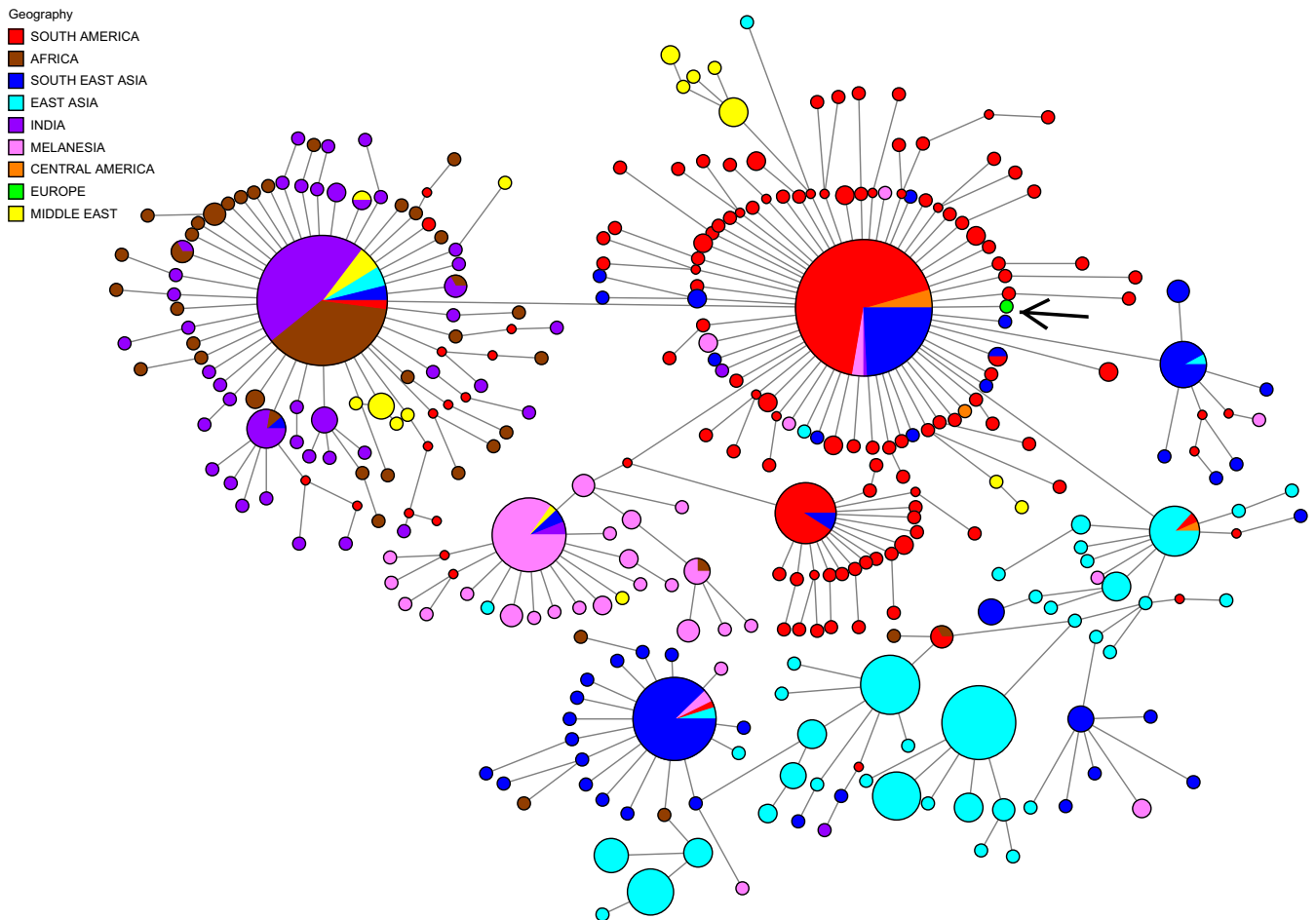
Fig. 2. Haplotype network constructed using NETWORK 5.0.0, incorporating 790 P. vivax mitochondrial DNA genomes previously published and the one retrieved in this study (arrow-marked European isolate). Size circles equal to the frequency of a given haplotype; lines separating haplotypes represent mutational steps. Each color shows the geographic origin of the samples.
