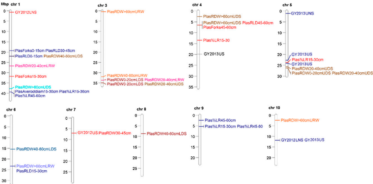
Figure 5. Chromosome map of significant loci for grain yield and root architectural plasticity detected under lysimeter and field conditions in the Aus 276 (blue shades) and Kali Aus (red shades) populations. LNS, Lowland nonstress; UNS, upland nonstress; US, upland stress; refer to Table I legend for other abbreviation definitions.
