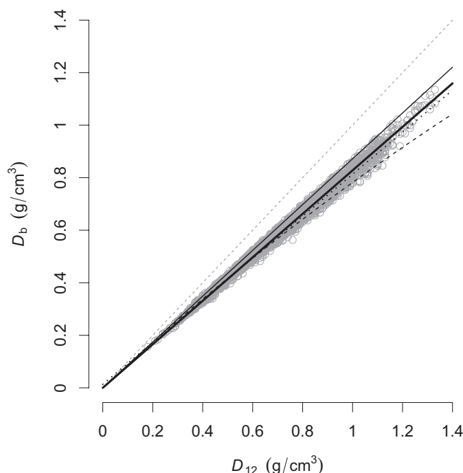
FIGURE 2. Relationship between basic wood density ( D_b oven dry mass/green volume, in \text{g/cm}^3 ) and wood density at 12% moisture ( D_{12} ). Gray dots represent the 3832 trees from the CIRAD database for which D_{12} , R , and S have been measured and D_b computed with our new formula. The gray dashed line represents the identity line. Based on D_{12} and D_b values, we estimated the following relationship (plain large black line): D_b = 0.828D_{12} ( n = 3832 , r^2 = 0.999 ). Using data and formula from Sallenave (1955, 1964, 1971), Chave et al. (2006) estimated a significantly different conversion factor of 0.872 (plain thin black line). We also plotted the relationships of Simpson (1993) (dashed black curve) and Reyes et al. (1992) (dotted black line).
