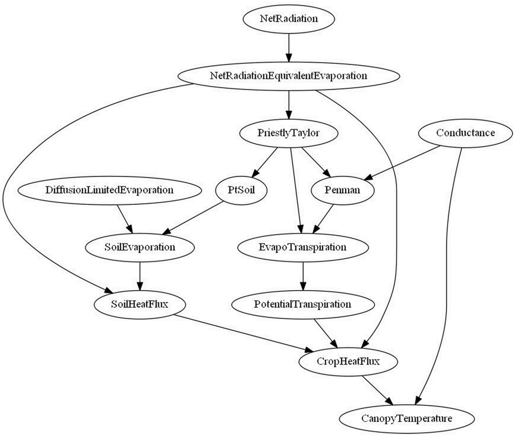
Fig. 9. Visualization of energy balance ModelComposite provided from SiriusQuality wheat model developed with the BioMA platform. Ellipses are ModelUnits and arrows represent the link between two ModelUnits.
