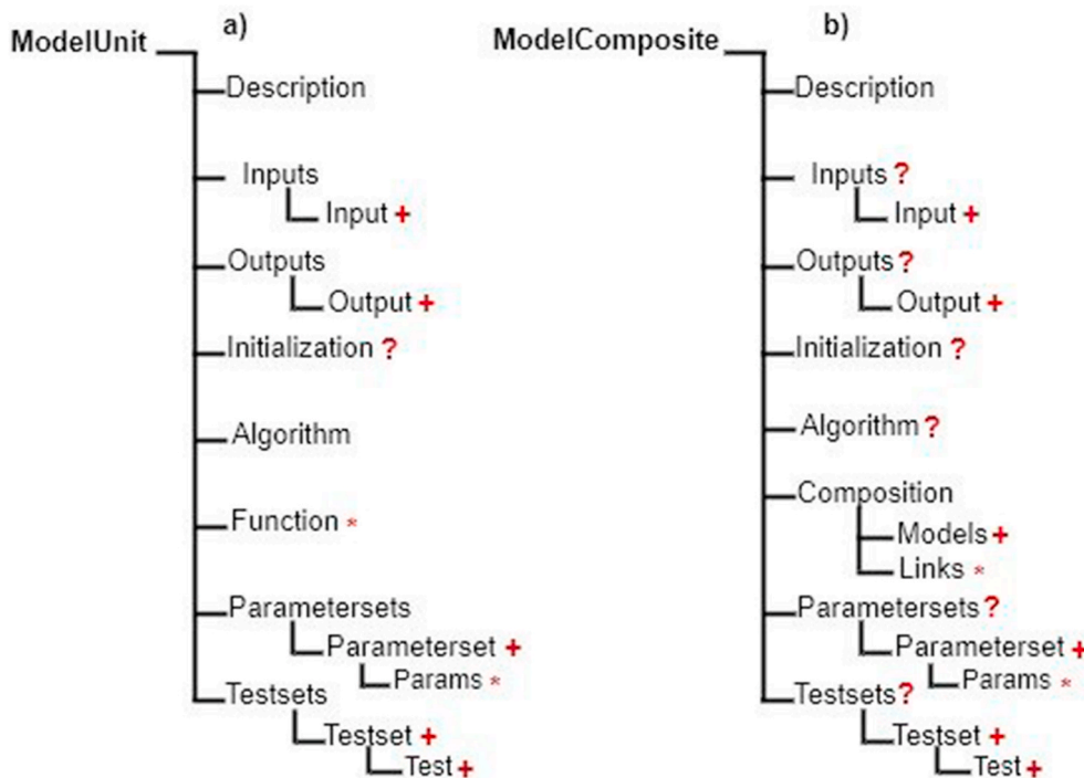
Fig. 2. Crop2ML concepts for model specifications: ModelUnit (a) and ModelComposite (b). “+”, one or more elements; “*”, zero or more elements; “?”, zero or one element.
