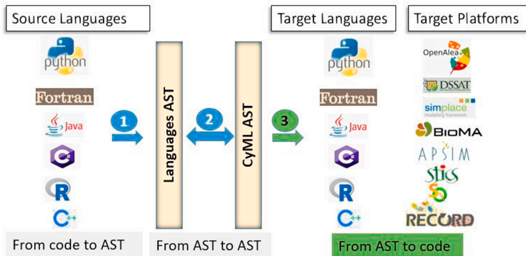
Fig. 11. Schema illustrating CyML transformation extensibility to support bidirectional source transformation.
