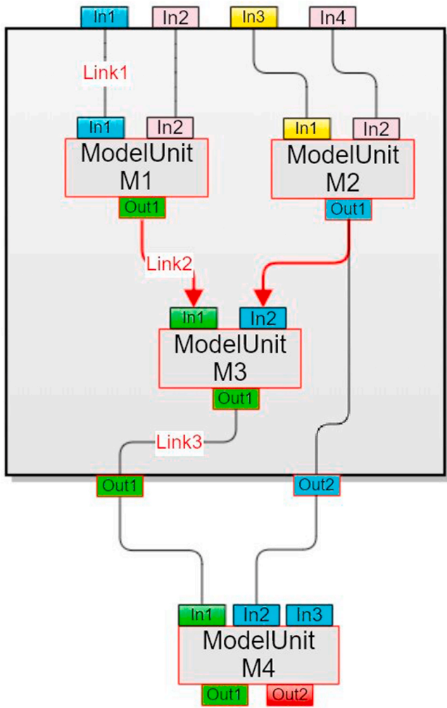
Fig. 7. Graph of a ModelComposite. Three ModelUnits (M1 to M3) are connected to form a first level of composition, which is linked to a fourth ModelUnit (M4). Link1 is an InputLink, Link2 is an InternalLink, and Link3 is an OutputLink. OutputLink is specified to clearly define the outputs of the ModelComposite, which necessarily include all state variables. Each model component has input ports In1, In2, ..., and output ports Out1, Out2, ..., where 1, 2, ..., are internal (local) port numbers.
