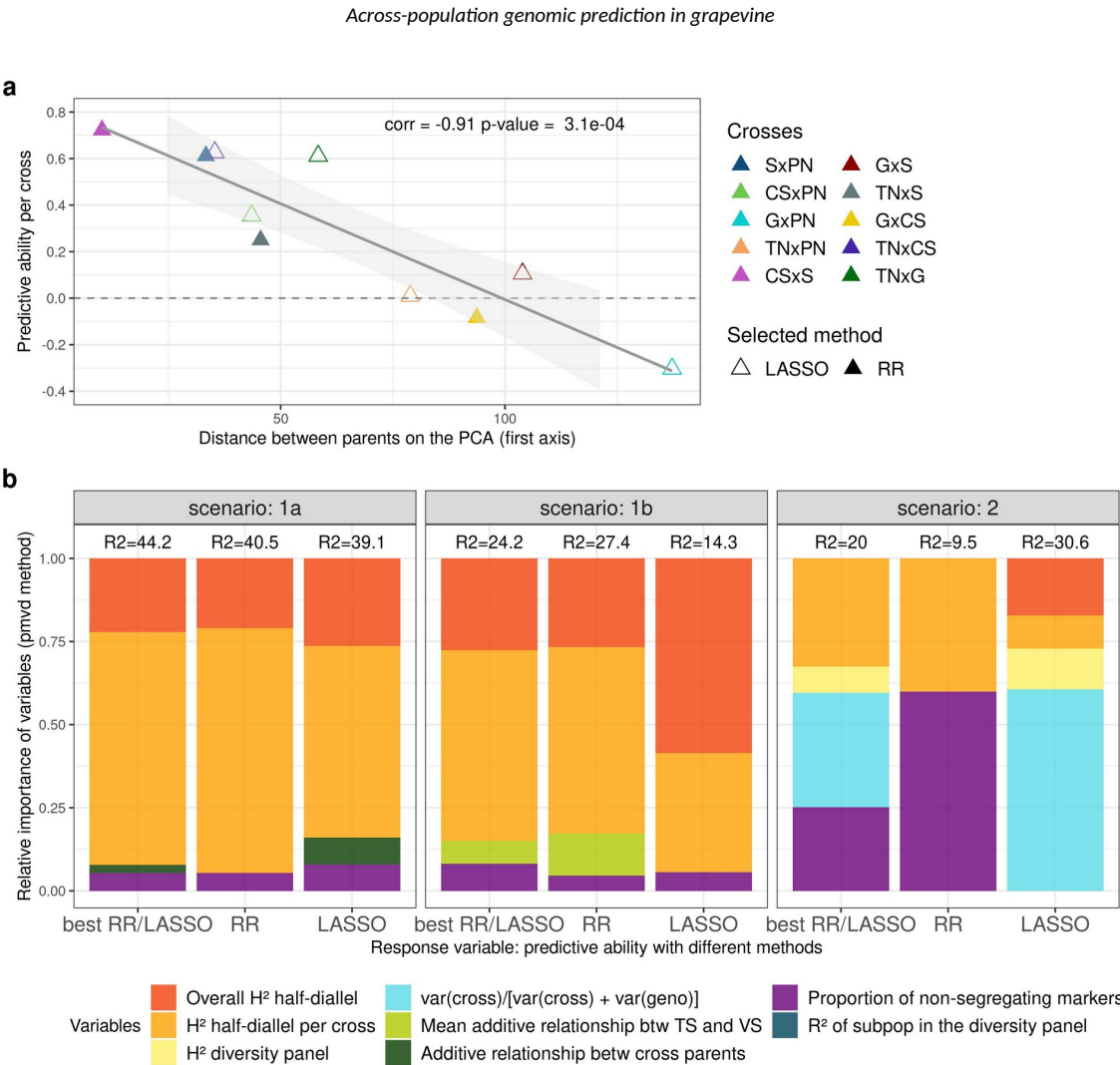
145 Figure 5: a: Plot of per-cross PA for cross mean in scenario 2, obtained with the best method between RR and LASSO for each cross, against the 146 distance between cross parents on the first axis of the diversity panel PCA (Figure 1a). Best method is indicated with the triangle filling and cross 147 with the color. b: Relative importance of variables affecting PA for Mendelian sampling in the three scenarios tested. Variables were selected 148 from an overall model, after a model selection step. Response individual PA values were obtained either as the best one between RR and 149 LASSO, with RR or with LASSO. Relative importance was estimated with pmvd method, from relaimpo R-package version 2.2-5.
