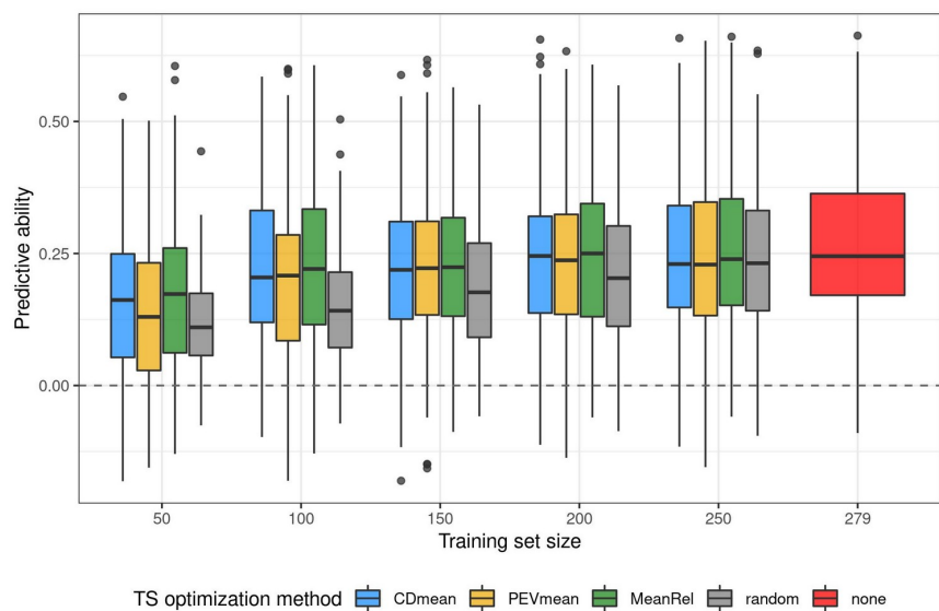
Figure S9 Distribution of predictive ability for Mendelian sampling genomic prediction, after training set optimization.
