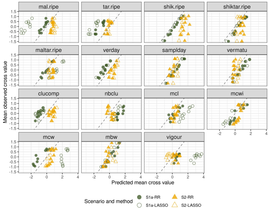
Figure S5 Observed vs predicted cross means for each trait in the half-diallel
