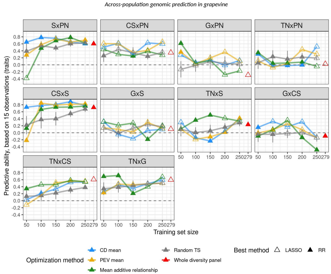
Figure 6: PA for cross mean prediction after training set optimization and with the best method between RR and LASSO, for each cross. Best method is indicated with the triangle filling and TS optimization method with the color. For comparison, random selection of TS genotypes (in grey) was performed and repeated ten times, error bars correspond to 95% of the confidence interval around the mean. We also report per-cross PA with the whole diversity panel (in red), with a maximum TS size of 279 which may vary depending on traits.
