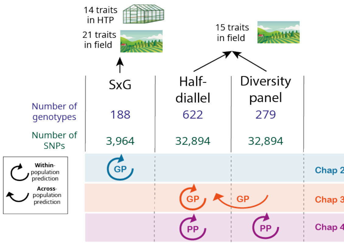
FIGURE 1.16 – Thesis outline.
