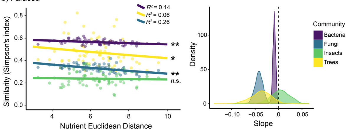
FIG. 4. Patterns of decay of similarity across nutrient distances and bootstrapped distribution of their slope for each community at (a) Nouragues and (b) Paracou. Dots represent pairs of plots, and lines are their fitted negative exponential functions. **, P < 0.01 ; *, P < 0.05 ; •, 0.05 < P < 0.10 ; and n.s., P \geq 0.10 .
