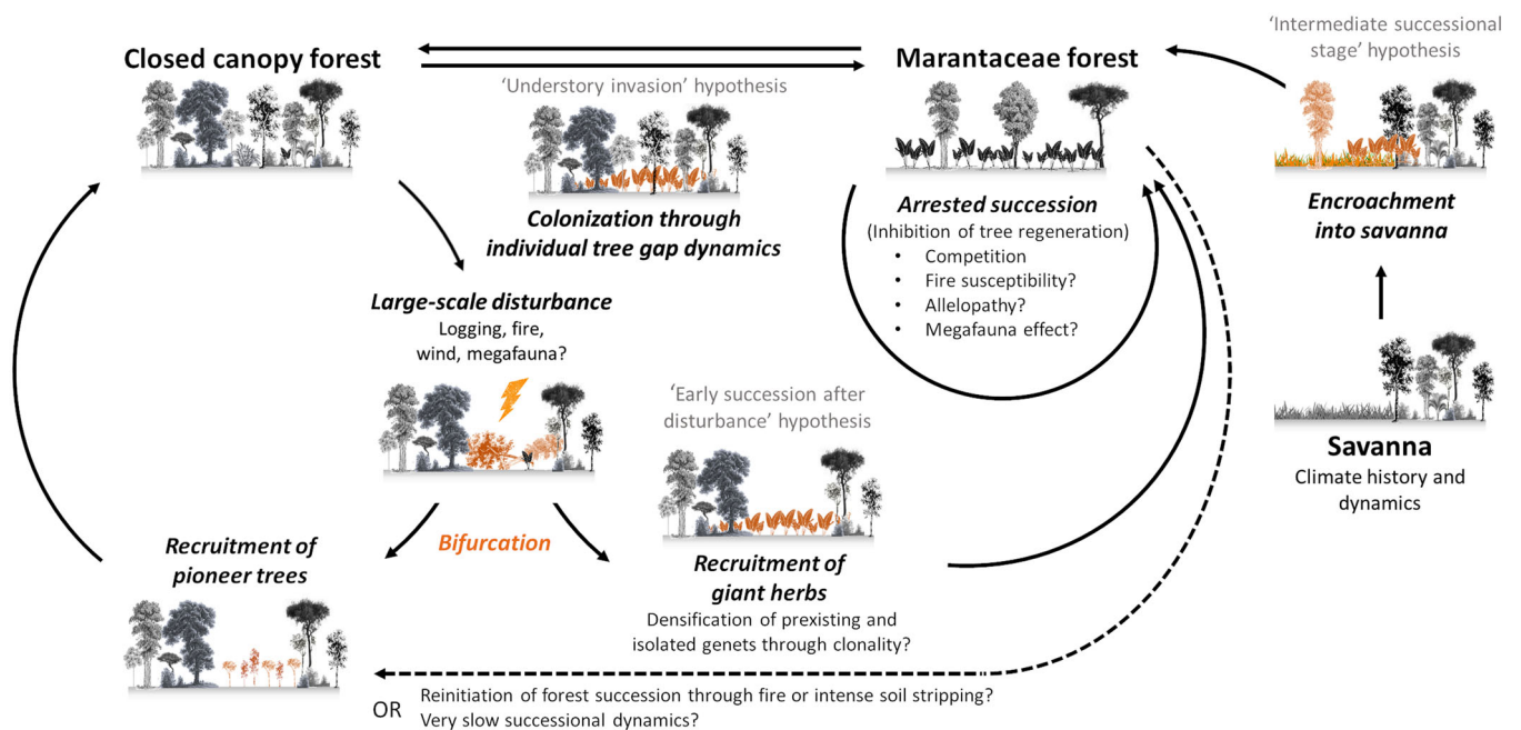
FIGURE 3 Summary of the ecological mechanisms that could be behind the local co-existence of Marantaceae forests and dense mixed-species forests in West-Central Africa. Arrows show the possible evolution of the system in different states. The three main hypotheses underlying the origin of Marantaceae forests are illustrated in the figure: (1) the ‘understory invasion’ hypothesis, where giant herbs gradually invade closed-canopy forests through natural tree fall gaps, (2) the ‘early succession after disturbance’ hypothesis, where giant herbs quickly invade the gaps after intense forest disturbances, and (3) ‘the ‘intermediate successional stage’ hypothesis, where giant herbs participate in the encroachment of savannas by forests and return slowly to a dense forest state.
