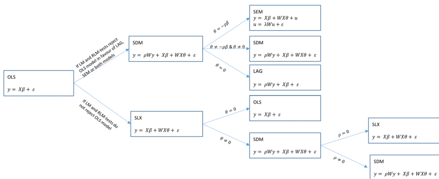
Fig. 2 Elhorst’s strategy to test for spatial spatial interaction effects on cross-sectional data
