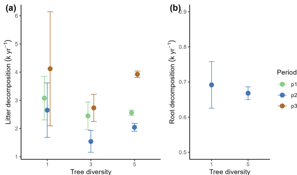
FIGURE 4 | Mean changes in leaf litter and root decomposition rates with time and diversity. Decomposition rates ( \text{k yr}^{-1} ) were calculated with a single-pool exponential decomposition model. Coloured points show means and error bars standard errors of the mean. The analyses considered three time intervals, early (p1), mid (p2) and late period (p3).
