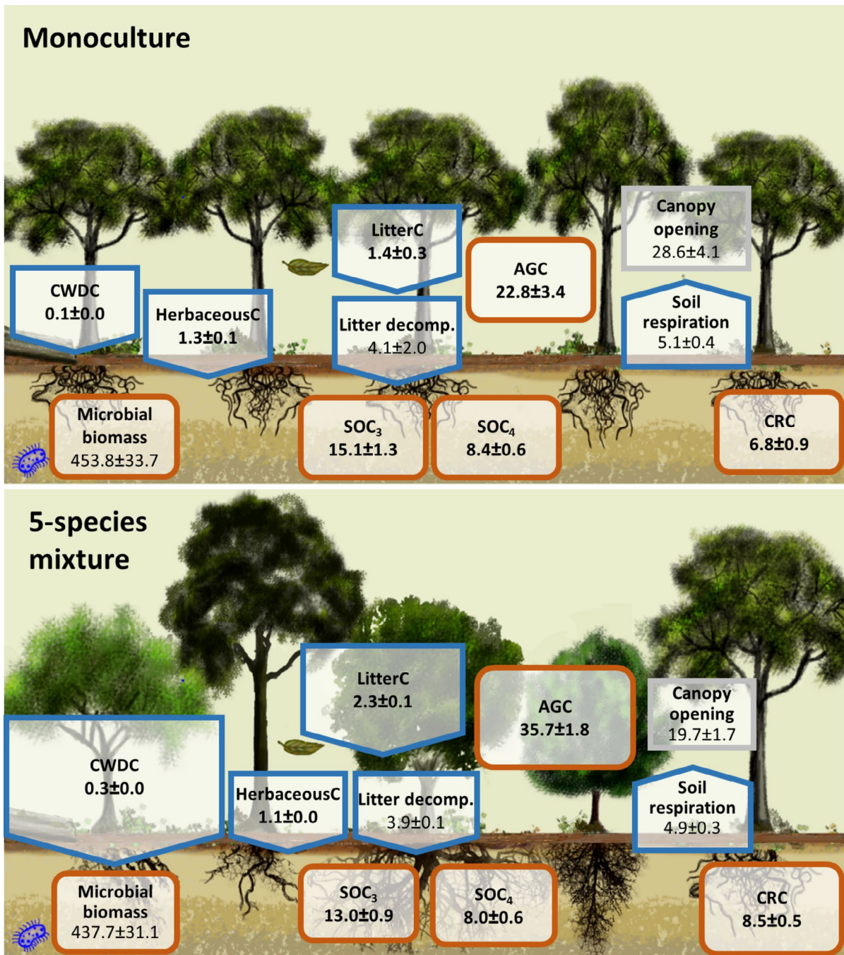
FIGURE 1 | C stocks and fluxes after 16 years of tree growth. Shown are means and standard errors of the C stocks in \text{Mg C ha}^{-1} (brown boxes) and fluxes in \text{Mg C ha}^{-1} \text{ year}^{-1} (blue arrows); numbers printed in bold. Variables in other units, including canopy opening in %, litter decomposition rate k \text{ year}^{-1} , soil respiration given in \mu\text{mol m}^{-2} \text{ s}^{-1} and microbial biomass given in \mu\text{g C}_{\text{mic}} \text{ g soil dw}^{-1} are not printed in bold to allow for separation. The size of the boxes and arrows in the 5-species mixture are scaled relative to the monoculture, with diversity-induced increases or decreases in C stocks and fluxes indicated by larger or smaller boxes/arrows, respectively. An overview of all analysed mixtures (2-, 3- and 5-species mixtures) is shown in Figure S4. The sum of \text{SOC}_3 and \text{SOC}_4 gives SOC. AGC, aboveground tree C; CRC, coarse root C; CWDC, coarse woody debris C; \text{SOC}_4 , \text{C}_4 derived soil organic C (SOC); \text{SOC}_3 , \text{C}_3 derived SOC.
