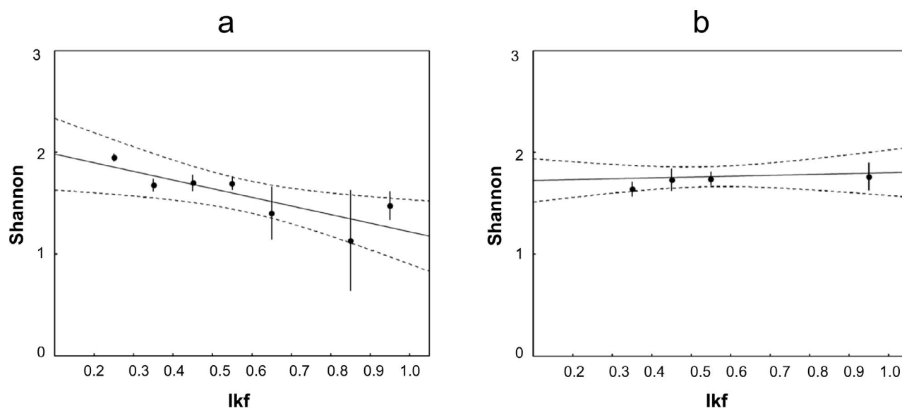
Fig. 5. Variations of bird species diversity (Shannon) in relation to wild boar foraging (lkf) and shrub density. Predicted trends are presented as black lines with 95% confidence intervals (dashed lines). Bars indicate the standard error + mean. a) bird species diversity in areas with low shrub cover. b) bird species diversity in areas with dense shrub cover.
