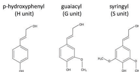
Figure 3: Lignin unit molecular structure
