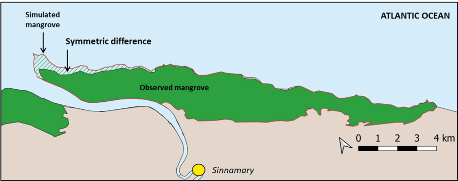
Fig. 5. Illustration of the symmetric difference of the simulated and observed mangrove areas for the Sinnamary sector. The calibration process attempts to minimize the magnitude difference. Sinnamary is located at 5.39°N and 52.96°W.
