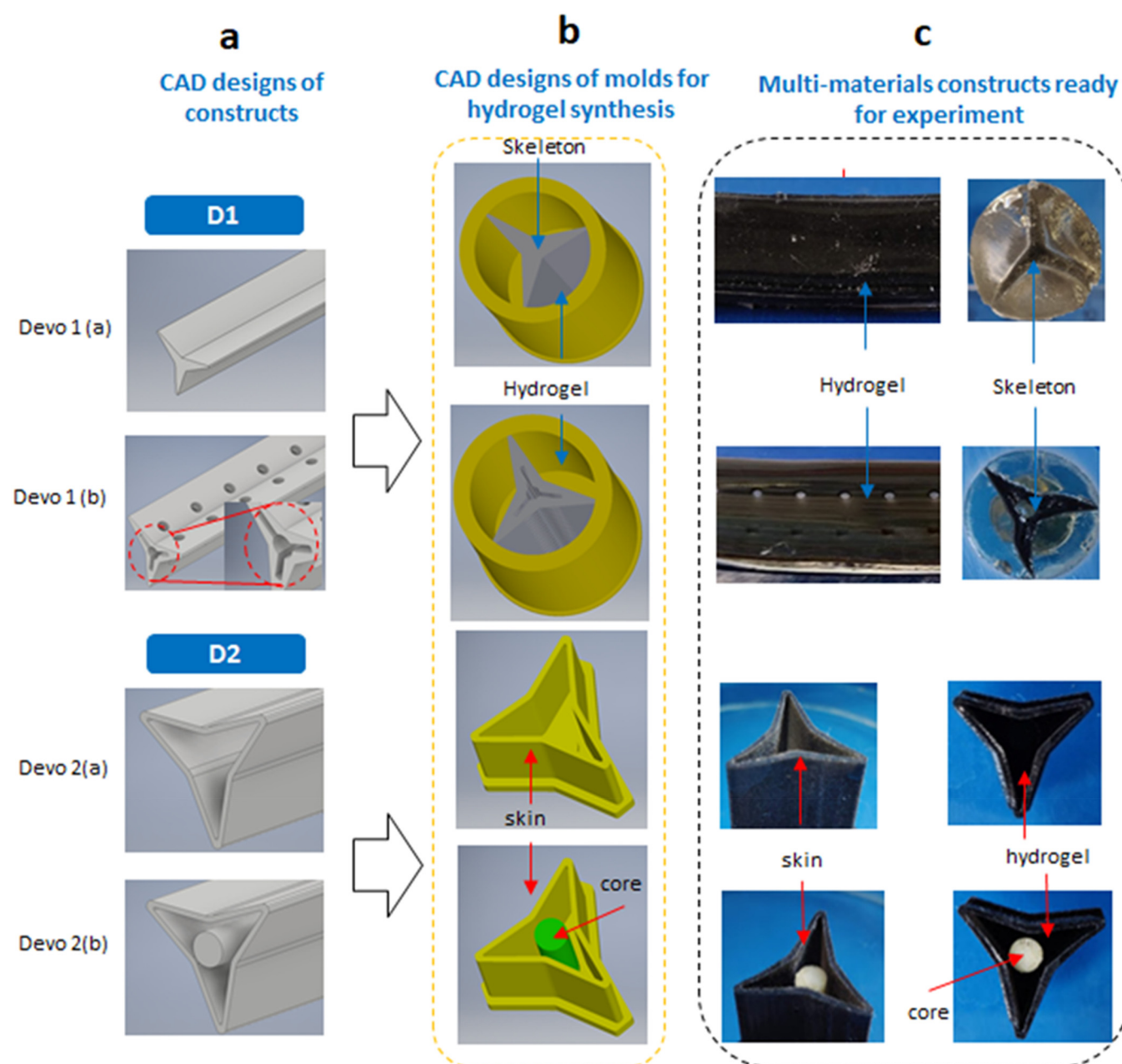
Fig. 3. CAD designs and fabrication method for two developmental designs. (a) CAD designs of solid (Devo 1(a)), porous (Devo 1 (b)) star-shaped skeletons and hollow thin star-shaped skin (Devo 2(a) and Devo 2(b)). (b) Hydrogel synthesis process at the different compartment of the solid skeleton (for D1) and within in the hollow skin (for D2). (c) Multi-material hydrogel-elastomer constructs for D1 (upper two rows) and artificial cactus for D2 (lower two rows). Panel a is the collection of CAD models of the actuator constructs. Panel b is the collection of CAD models of the mould, where 3D printed constructs are inserted into the mould for hydrogel synthesis for Devo 1 and 3D printed constructs act as mould themselves for Devo 2. Panel c is the collection of the developed multi-material constructs ready for the actuation experiment.
